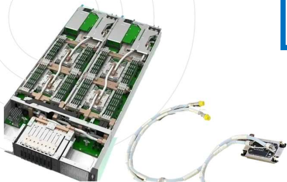
Cold Plate Modules
