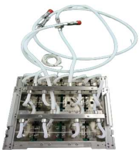
GPU Cold Plate
